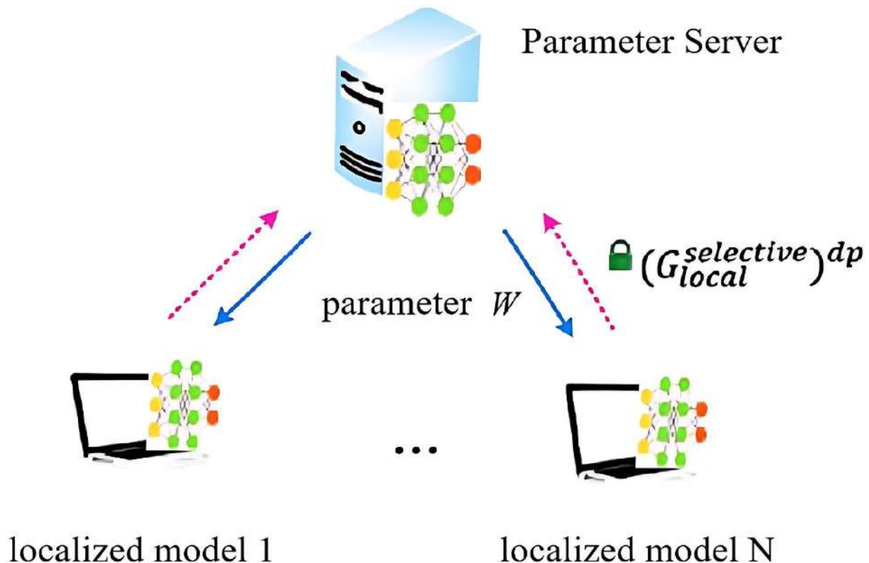
Figure 4. Framework for DSSGD.
