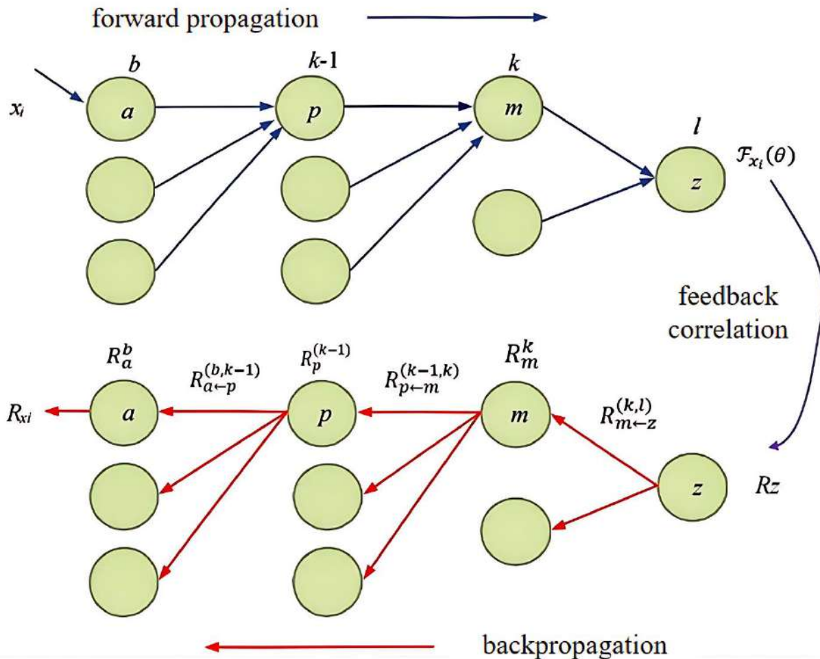
Figure 5. Framework for LRP.
