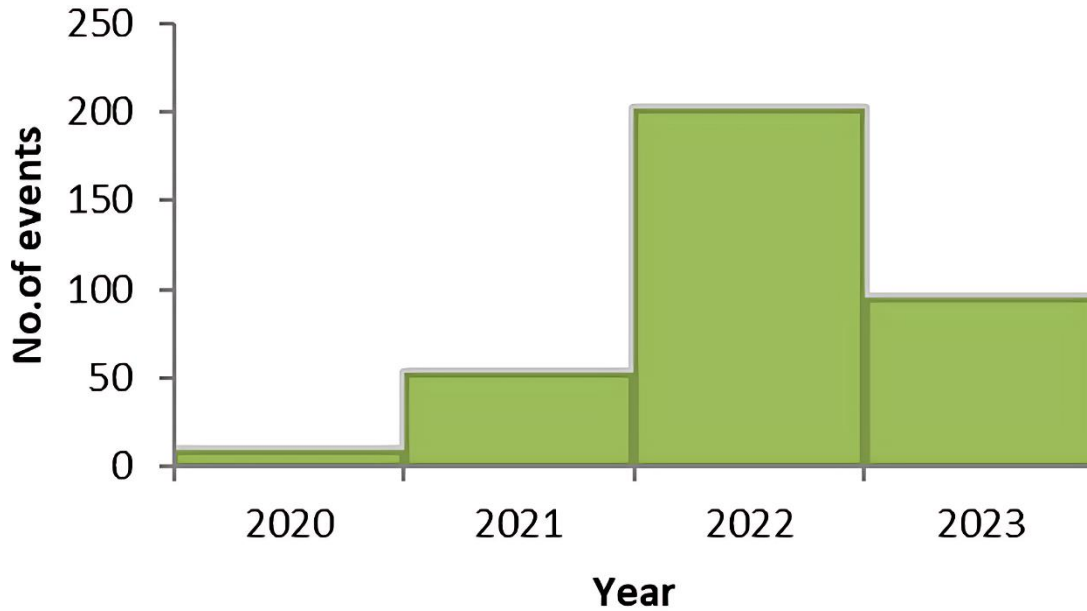
Figure 3. Represent number of strong normal CMEs with years at CS25.
