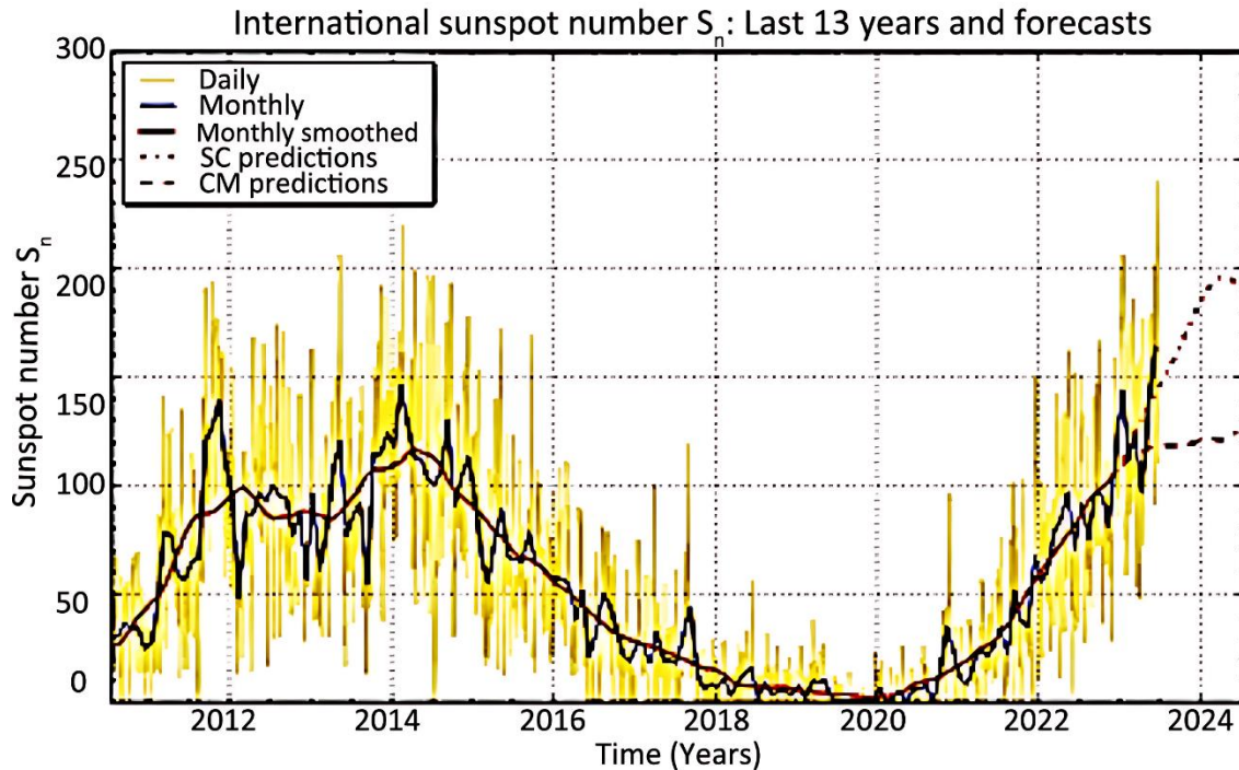
Figure 1. Sunspot numbers with time at solar cycle 24 and beginning of solar cycle 25 ( http://sidc.be/silso ) Royal Observatory of Belgium 2023 July.
