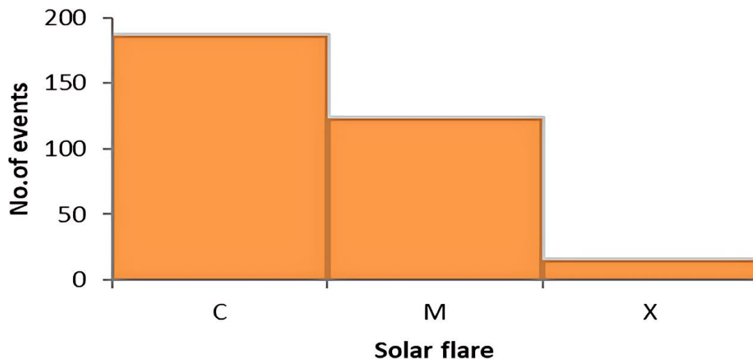
Figure 2. Represent the number of Solar flares with magnitude amount of its during present study time.
